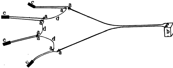
Fig. 18. Method of Blasting Several Stumps at Once; b Represents Electric Blasting Machine; c a Charge of a Stump Connected by the Cap-Wire into the Circuit at a; d Represents an Insulated Wire Connecting One Charge with Another
